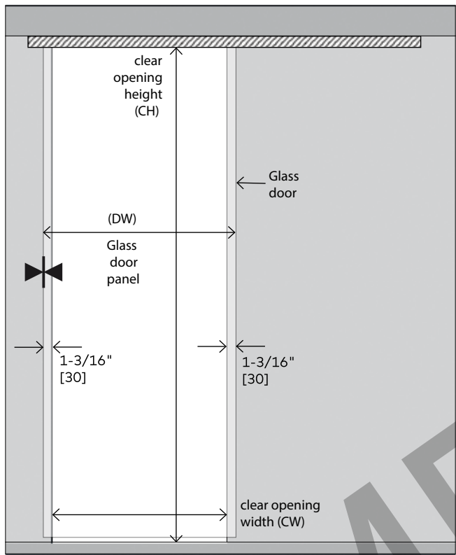
Single door mount
